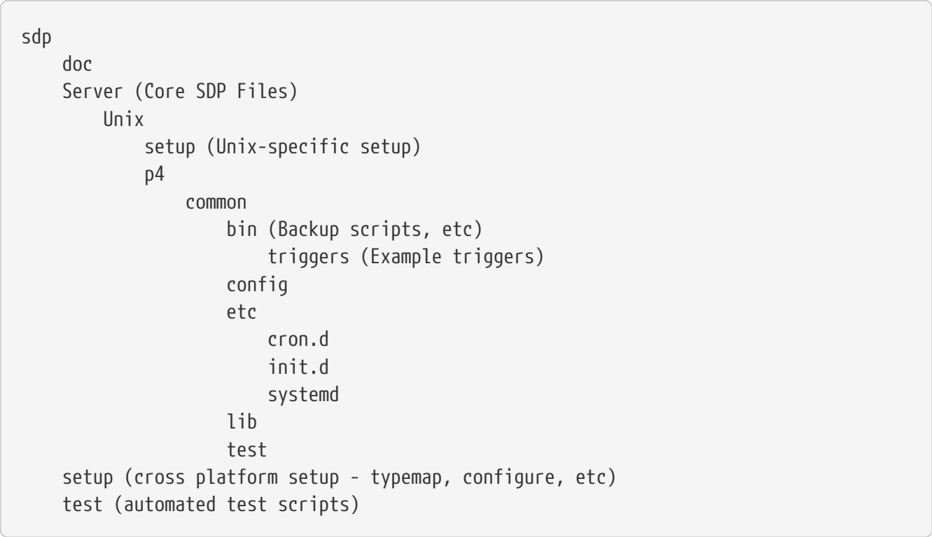
Figure 1 - SDP Package Directory Structure
